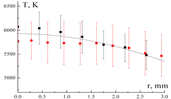
Figure 1. Radial distribution of plasma temperature, arc current 3.5 A ■ –monochromator, ● –spectrograph.
