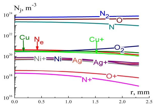
Figure 14. Equilibrium plasma composition for arc current 3.5 A obtained with copper vapors density, plasma temperature and relative intensities of Cu I, Ag I, Ni I spectral lines.
