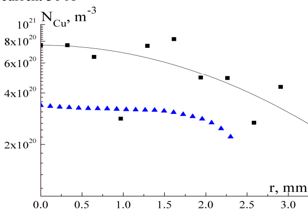
Figure 5. Radial distribution of copper vapor density in plasma, arc current 3.5 A: ■ – Laser Absorption Spectroscopy (LAS); ▲ – obtained from calculation of equilibrium plasma composition.
