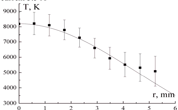
Figure 3. Radial distribution of plasma temperature, arc current 30 A.
