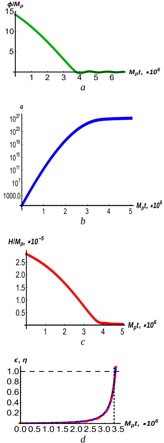
Fig. 2. Time dependencies of the inflation field (a), scale factor (b), Hubble parameter (c) and slow-roll parameters \epsilon and \eta (d). The used axion decay constant f = 7.5M_p , corresponds to \Lambda = 1.4 \times 10^{16} \text{ GeV} .
