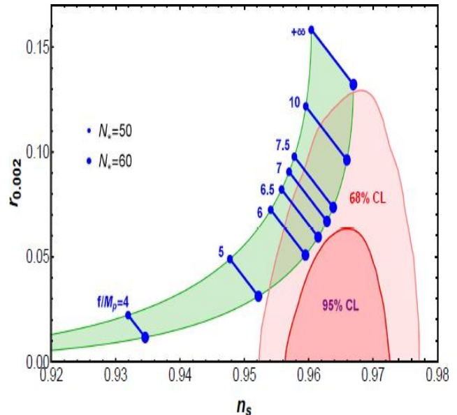
Fig. 6. Theoretical prediction for n_s and r from natural inflation model (region between two growing curves) for 50 < N_* < 60 and 0 < f/M_p < \infty , and marginalized joint 68 CL and 95% CL regions for n_s and r at k_* = 0.002 Mpc^{-1} [3].
