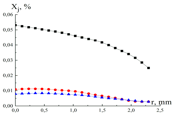
Figure 15. Content of metal vapors in the arc discharge plasma, current 3.5 A: ■ – Cu, ● – Ag, ▲ – Ni (determined with the using of T(r) and N_e(r) , without account of \text{NO}^+ ).
