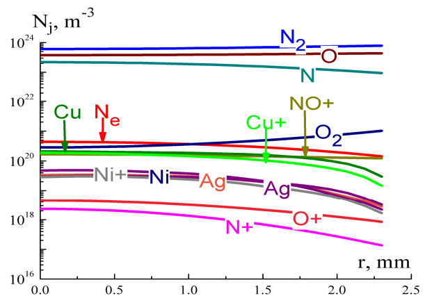
Figure 12. Equilibrium plasma composition for arc current 3.5 A obtained with electron density, plasma temperature and relative intensities of Cu I, Ag I, Ni I spectral lines.
