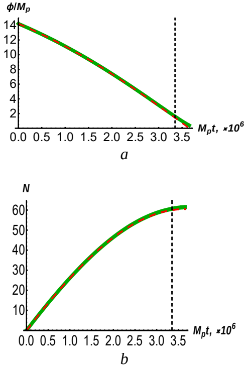
Fig. 3. Time dependencies of the inflation field and scale factor (number of e-folds) obtained from numerical integration of the system of Friedmann and KGF equations (solid lines a , b ) and approximate analytical solutions (165) and (166) derived in a slow-roll approximation. Vertical dashed line shows the moment of the end of inflation when \epsilon = 1 .
