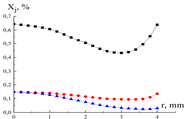
Figure 11. Content of metal vapors in the arc discharge plasma, current of 30 A: ■ – Cu, ● – Ag, ▲ – Ni (determined with the using of T(r) and N_e(r) , with account of NO^+ ).
