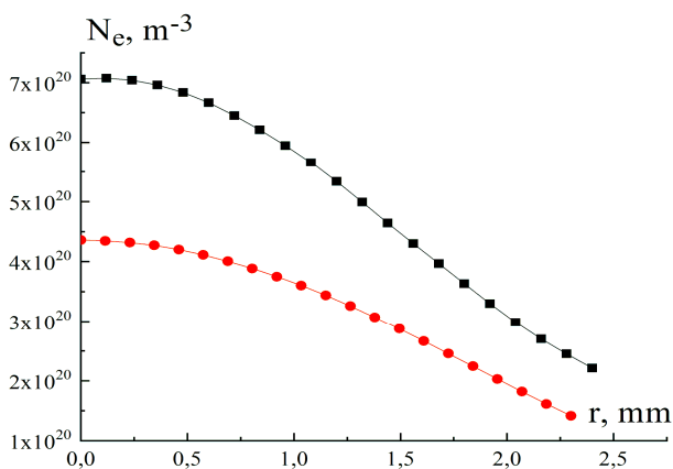
Figure 6. Radial distribution of electron density in plasma, arc current 3.5 A (● – obtained from energy balance equation; ■ – obtained by LAS and equilibrium plasma composition calculation).
