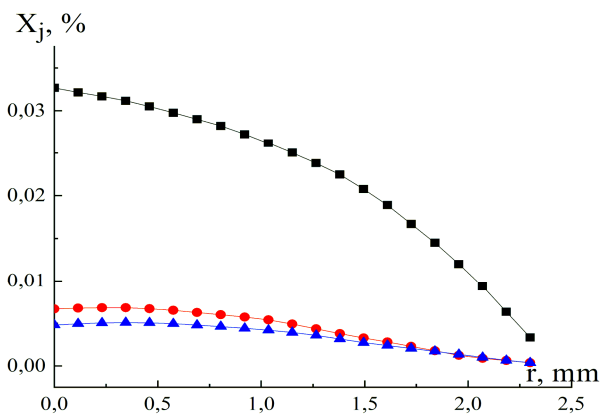
Figure 13. Content of metal vapors in the arc discharge plasma, current 3.5 A: ■ – Cu, ● – Ag, ▲ – Ni (determined with the using of T(r) and N_e(r) , with account of NO^+ ).
