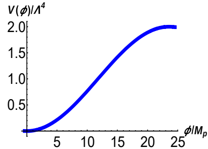
Fig. 1. The inflation potential (163) in the natural inflation model for the decay constant f = 7.5M_p .
