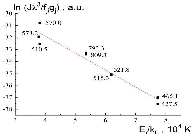
Figure 4. Boltzmann plot of Cu I ( r=0 mm), arc current 30 A
