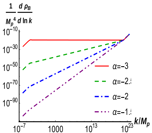
Fig. 4. Square modulus of the mode function and magnetic power spectrum at the end of inflationary stage for different values of \alpha .
