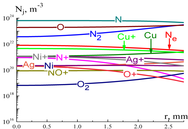
Figure 10. Equilibrium plasma composition for arc current 30 A obtained with electron density, plasma temperature and relative intensities of Cu I, Ag I, Ni I spectral lines.
