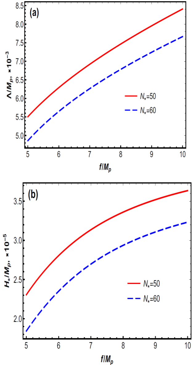
Fig. 7. The parameter \Lambda (panel a) and the Hubble parameter at the moment of the pivot scale horizon crossing H_* (panel b) as functions of f for fixed N_* = 50 (solid lines) and N_* = 60 (dashed lines) obtained from Eqs. (198).
