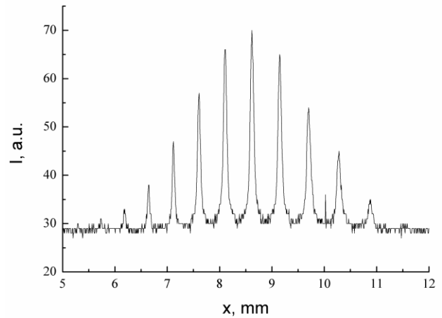
Figure 7. Registered interferogram of spectral line Ag I 447.6 nm.
