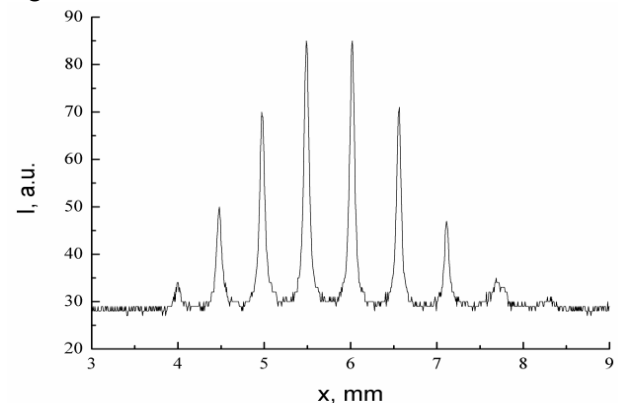
Figure 8. Registered interferogram of spectral line Cu I 515.3 nm.
