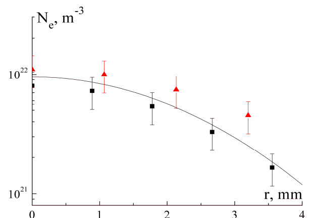
Figure 9. Radial distributions of electron density in plasma, arc current 30 A, obtained from half-width of spectral lines ▲ – Cu I 515.3 nm, ■ – Ag I 447.6 nm.
