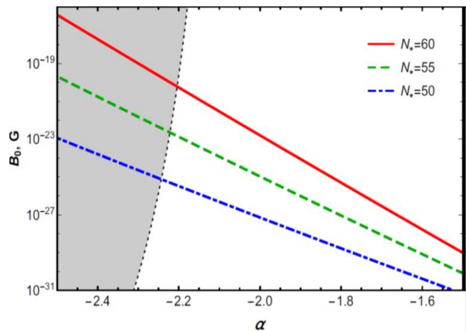
Fig. 5. The present day value of the magnetic field as a function of \alpha for different number of e-folds N_* = 50, 55, 60 .
