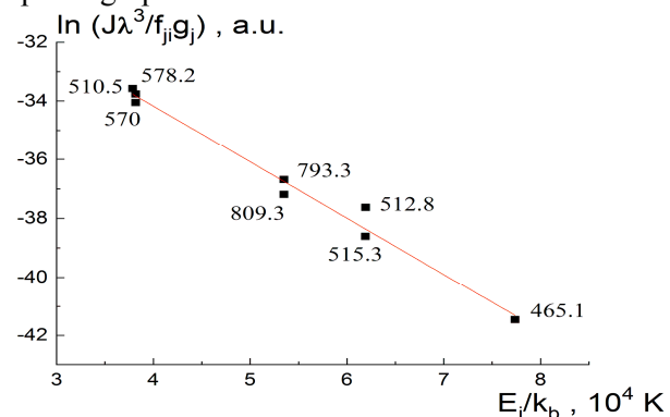
Figure 2. Boltzmann plot of Cu I ( r=0 mm), arc current 3.5 A
